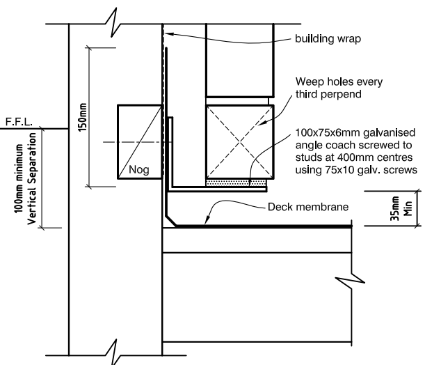
FIG.10 ENCLOSED DECK
